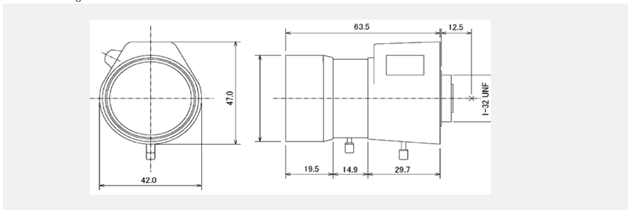
Dimension drawing
