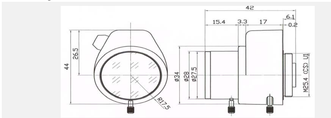
Dimension drawing
